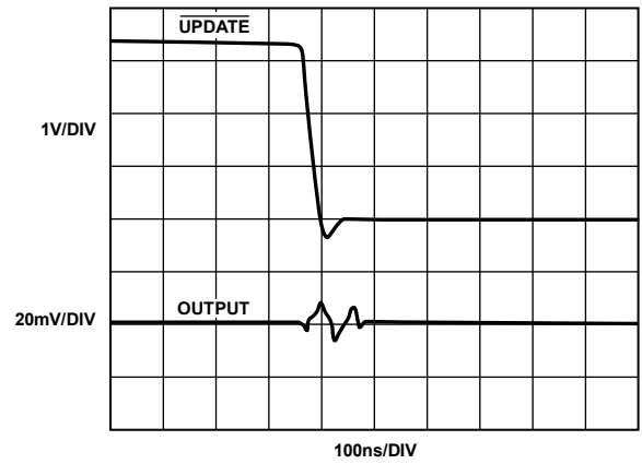
Figure 23. Switching Transient
