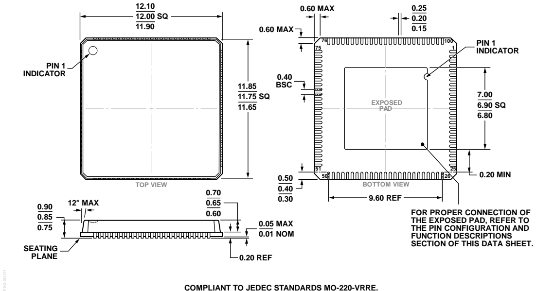
COMPLIANT TO JEDEC STANDARDS MO-220-VRRE. Figure 66. 100-Lead Lead Frame Chip Scale Package [LFCSP_VQ] 12 mm × 12 mm Body, Very Thin Quad (CP-100-1) Dimensions shown in millimeters
