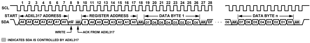
Figure 3. I 2 C Multibyte Register Write
