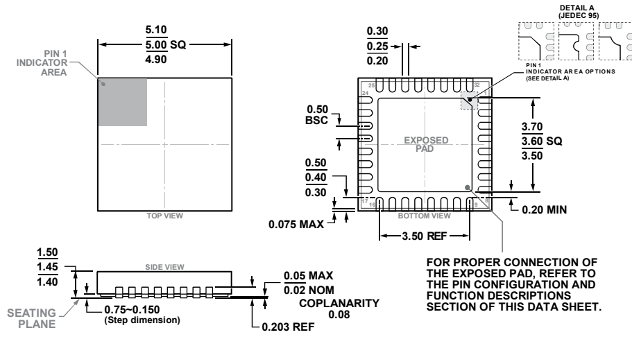
Figure 41. 32-Lead Frame Chip Scale Package [LFCSP_SS] 5 mm × 5 mm Body and 1.45 mm Package Height, with Side Solderable Leads (CS-32-4) Dimensions shown in millimeters
