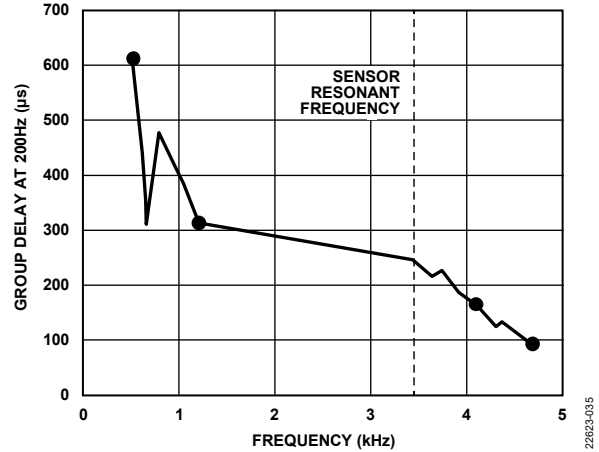
Figure 35. Z-Axis Group Delay vs. Frequency for All Filter Settings (See Table 15 for Specific Items in This Figure Marked with Circles)
