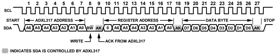
Figure 2. I 2 C Single-Byte Register Write
