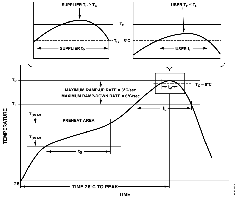
Figure 38. Pb-Free Solder Profile
