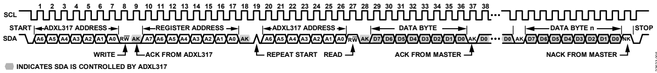
Figure 5. I 2 C Multibyte Register Read
