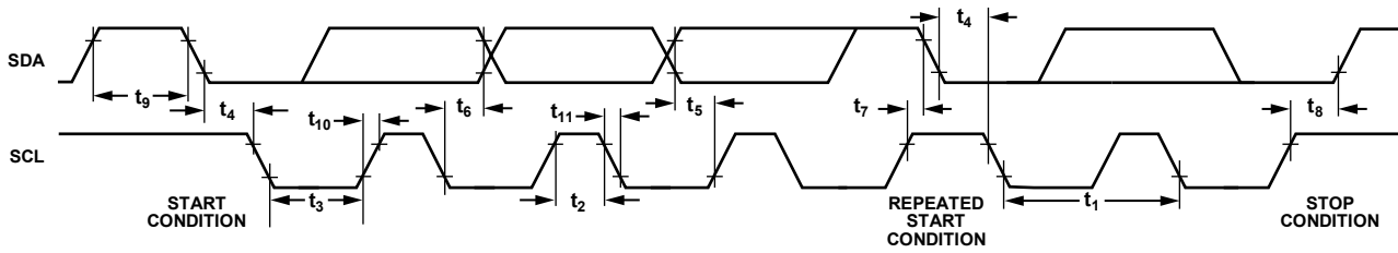
Figure 6. I 2 C Timing Diagram
