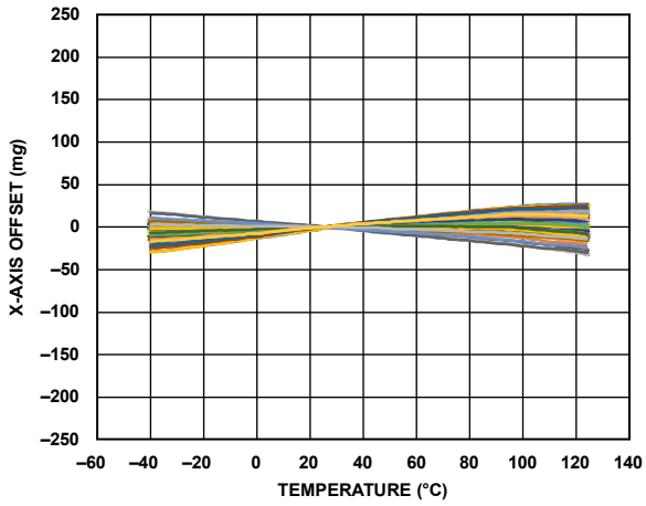
Figure 8. X-Axis Offset vs. Temperature
