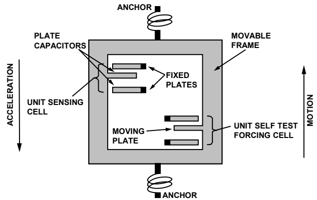
Figure 20. Simplified View of One Sensor During Acceleration
