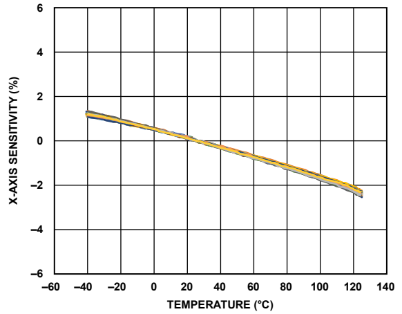
Figure 11. X-Axis Sensitivity vs. Temperature (500 Hz Cascaded Filter)
