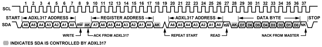
Figure 4. I 2 C Single-Byte Register Read
