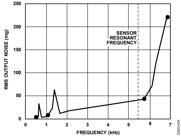
Figure 34. X- and Y-Axes Noise vs. Frequency for All Filter Settings (See Table 15 for Specific Items in This Figure Marked with Circles)
