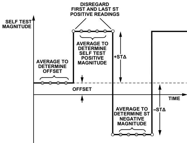
Figure 24. AC Self Test Measurement
