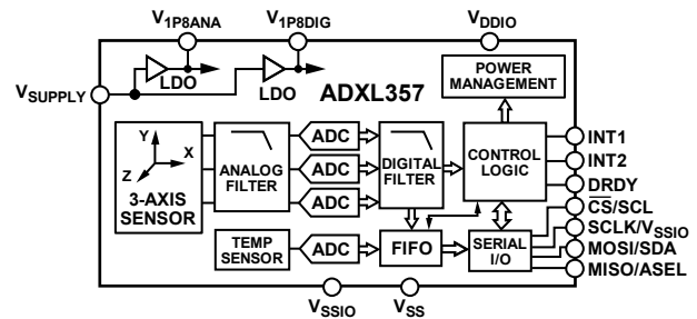
Figure 2. ADXL357
