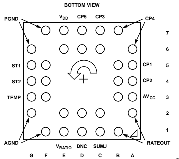
Figure 3. Pin Configuration
