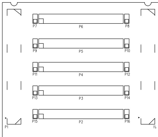
Figure 2-1. Connector Locations
