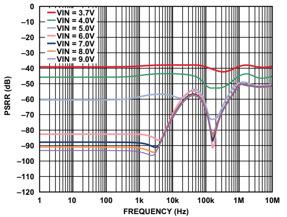
Figure 8. V_{\text{OUT2}} PSRR, I_{\text{VOUT2}} = 50\ \text{mA}
