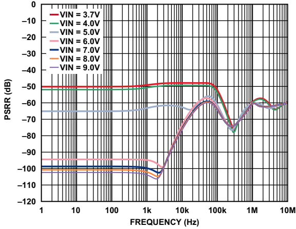
Figure 5. V_{\text{OUT1}} PSRR, I_{\text{VOUT1}} = 10\ \text{mA}
