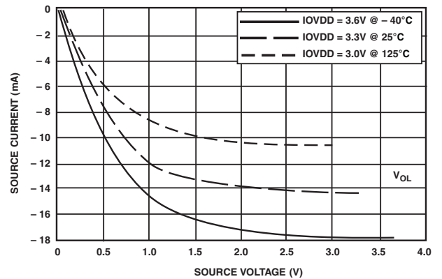
Figure 23. \bar{P} C Drivers (3.3 V IOVDD)
