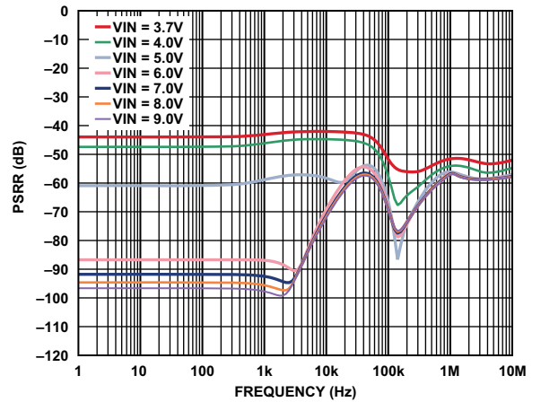
Figure 7. V_{\text{OUT2}} PSRR, I_{\text{VOUT2}} = 10\ \text{mA}
