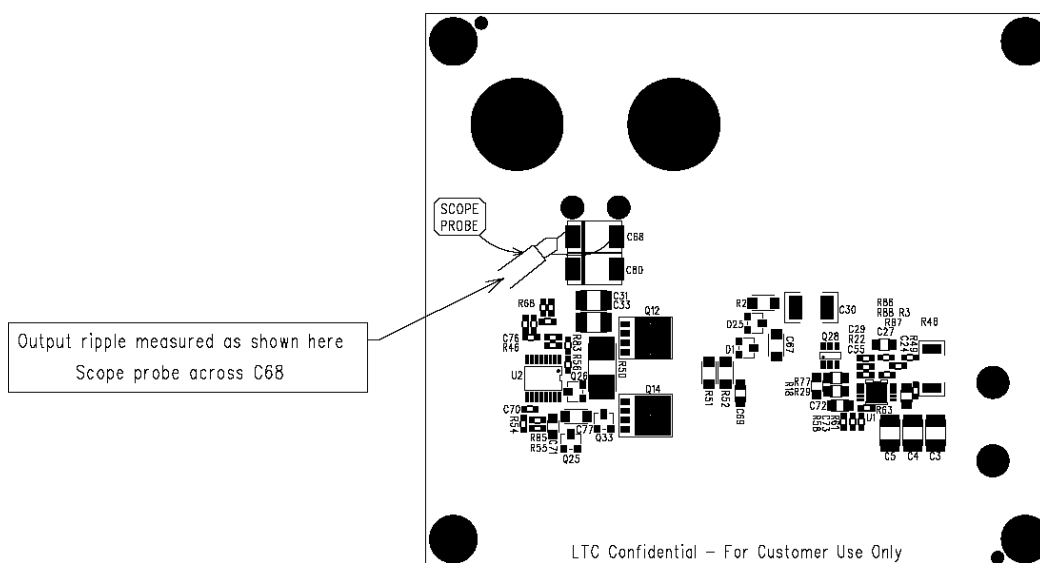
Figure 2. Measuring Input or Output Ripple
