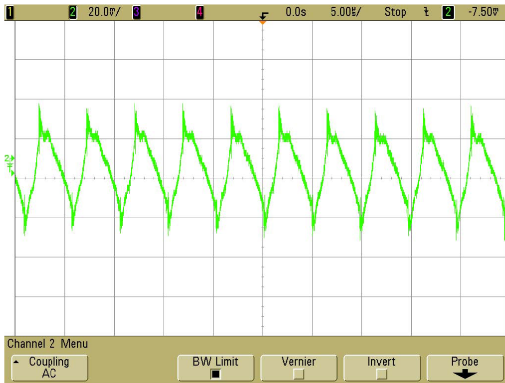
Figure 4. Output Ripple at 18Vin and 20Aout (25MHz) (20mV, 5us / div, 25MHz)
