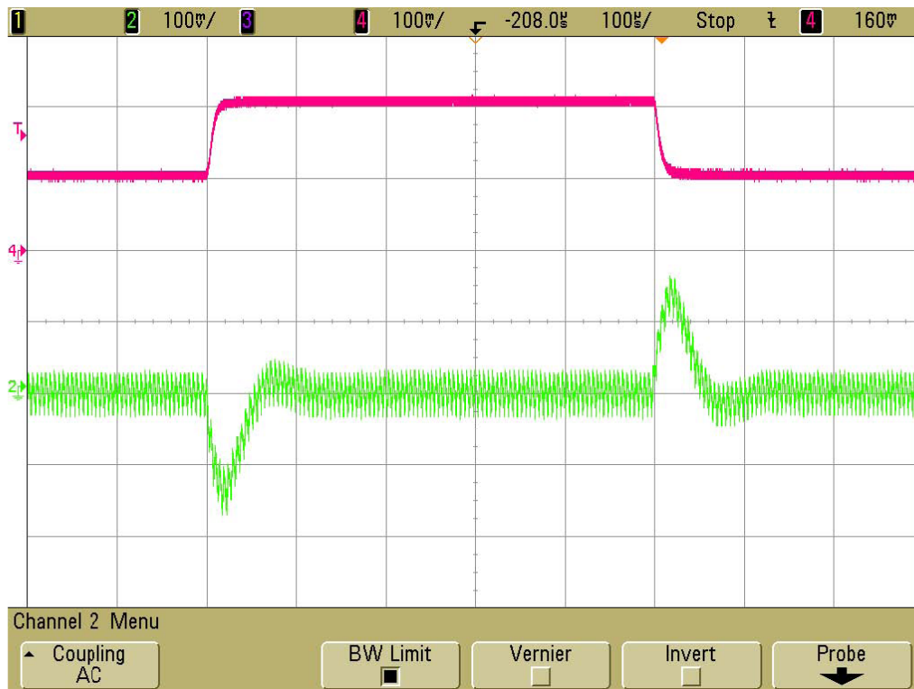
Figure 5. Transient Response Waveform at 18Vin and 10 - 20Aout (10A, 1000mV, 100us / div)
