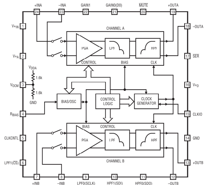
The LTC6602 BLOCK DIAGRAM
