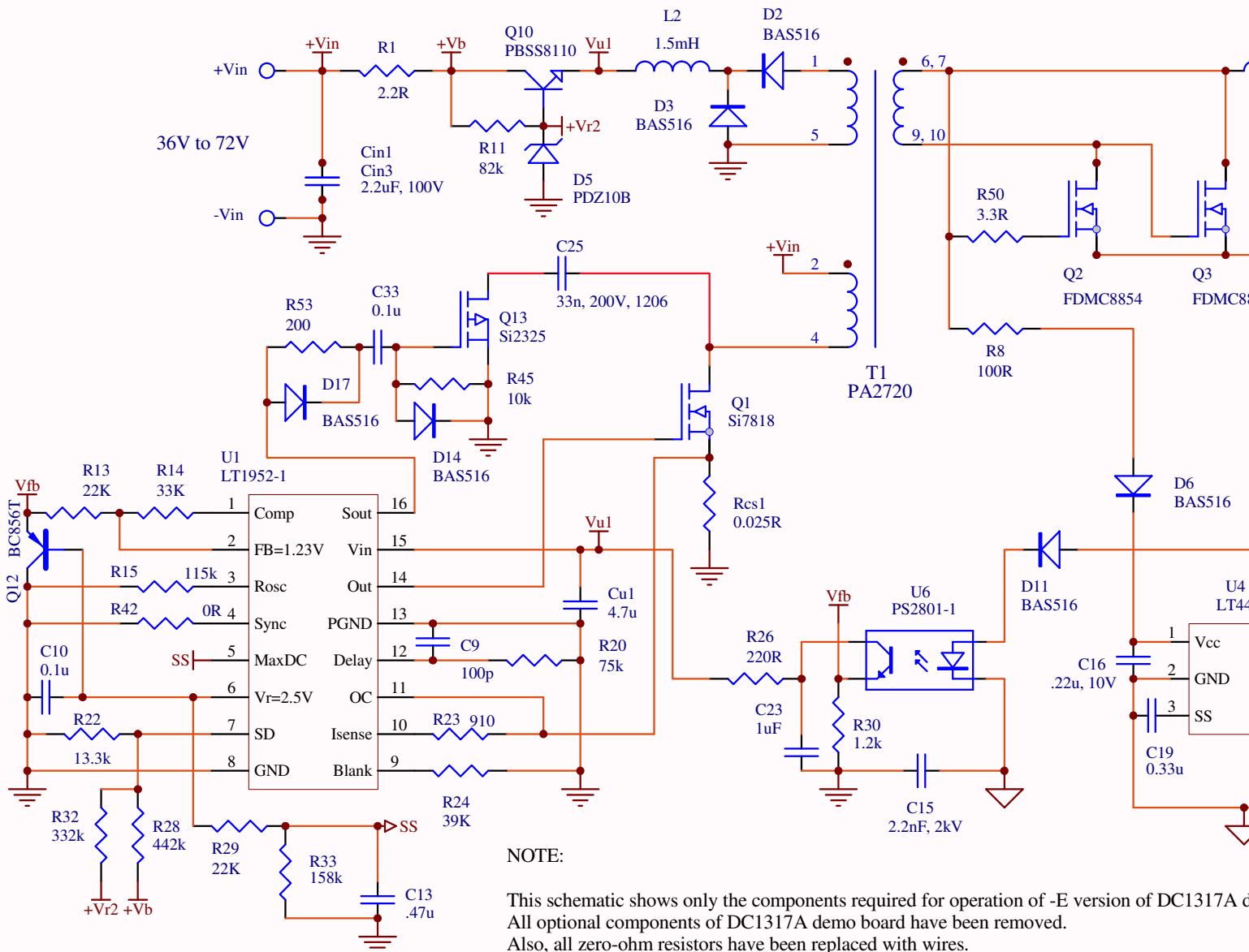
DC1317A-E schematic
