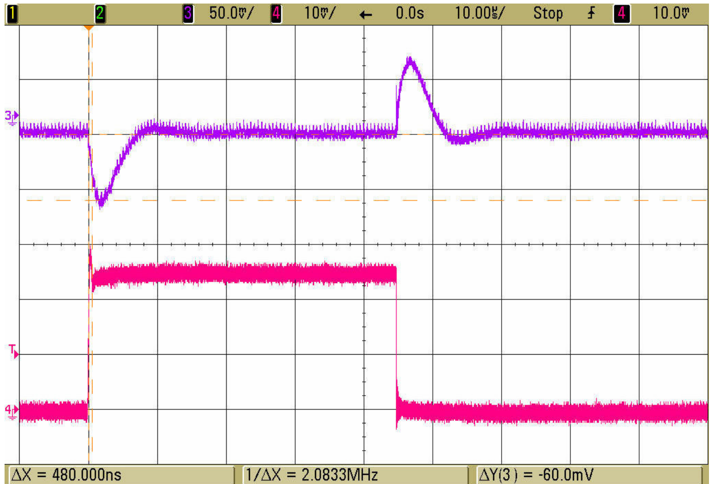
Figure 4. Load Step Response V_{IN} = 12\text{V} , V_{OUT} = 1.8\text{V} , 2.5A Load Step (0A \leftrightarrow 2.5A) Forced Continuous Mode F_{SW} = 2\text{MHz} Trace 3: Output Voltage (50mV/div AC) Trace 4: Output Current (1A/div)
