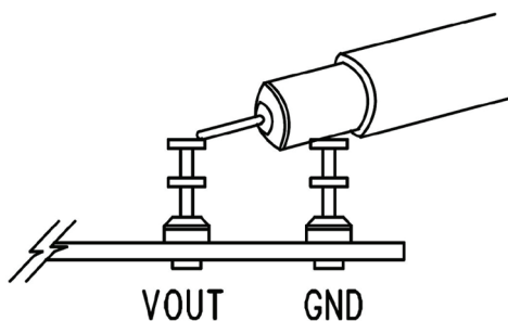
Figure 3. Measuring Output Ripple
