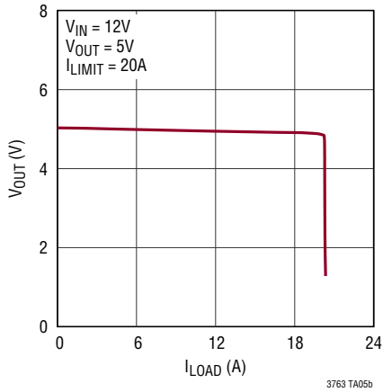
Output Voltage Load Regulation
