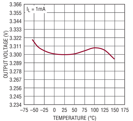
Output Voltage—LT3055-3.3
