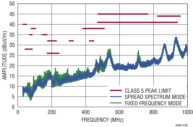
Radiated Peak
