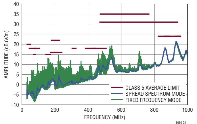
Radiated Average
