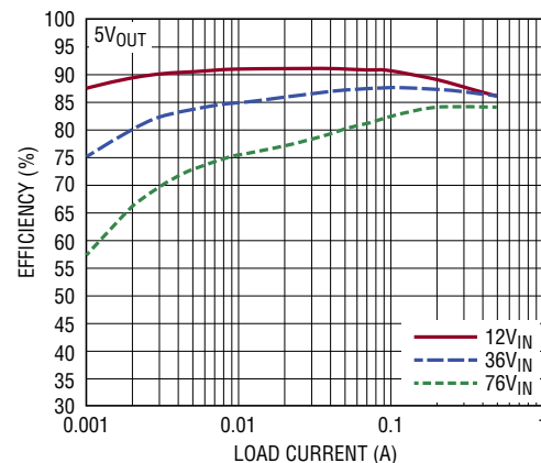
Figure 3. Efficiency Curves
