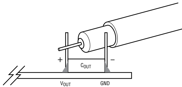
Figure 2. Measuring Output Ripple
