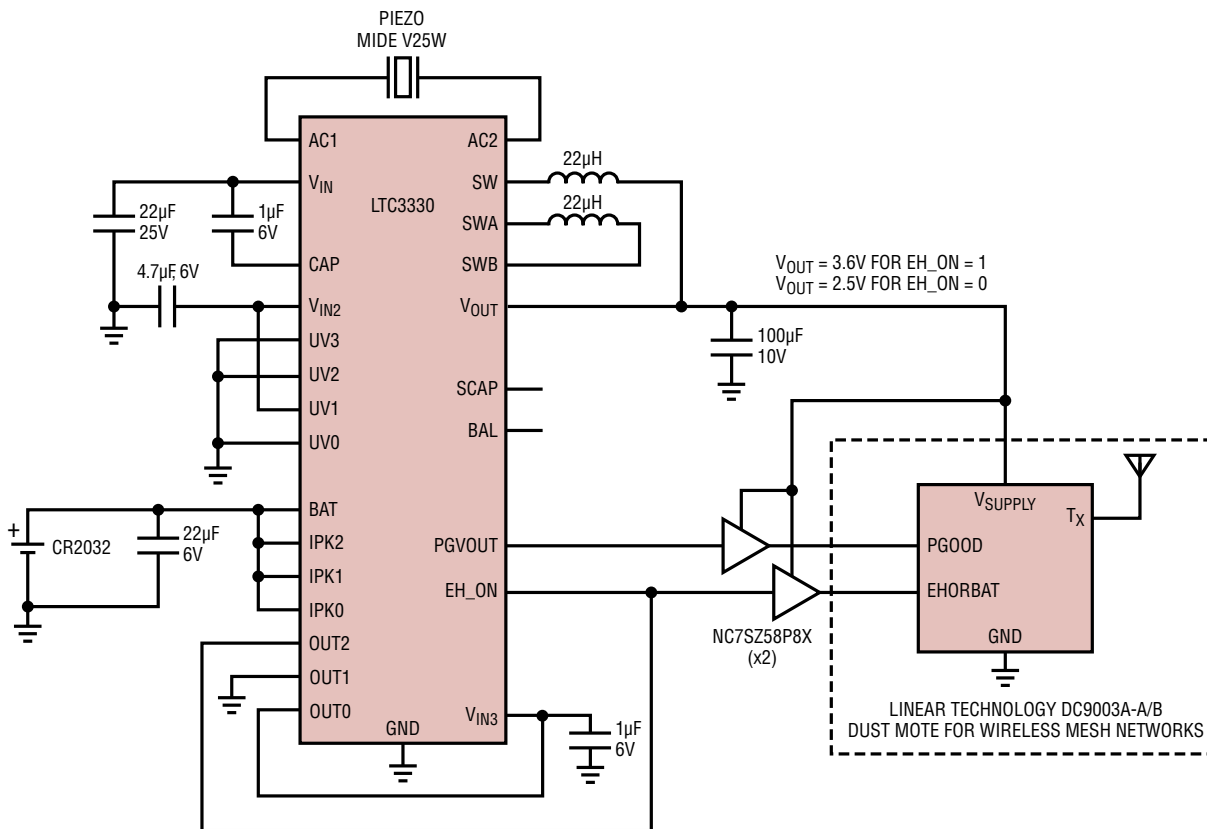
Figure 15. Dust Mote Setup without a Supercapacitor and with EH_ON Connected to OUT2
