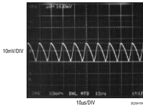
Figure 4. Output Voltage Ripple for the LT1676, I_L = 500mA
