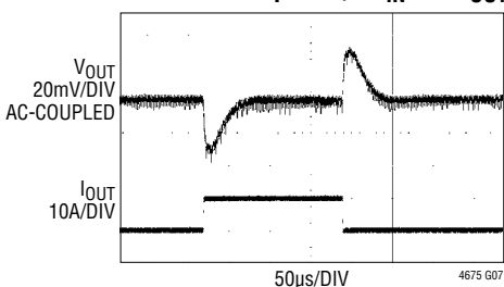
FIGURE 27 CIRCUIT AT 5\text{V}_{\text{IN}} . \text{VOUT\_COMMAND}_n SET TO 1.000\text{V} . 8A TO 18A LOAD STEP AT 10\text{A}/\mu\text{s}
