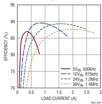
-15V Efficiency vs Load Current
