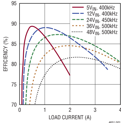
-3.3V Efficiency vs Load Current
