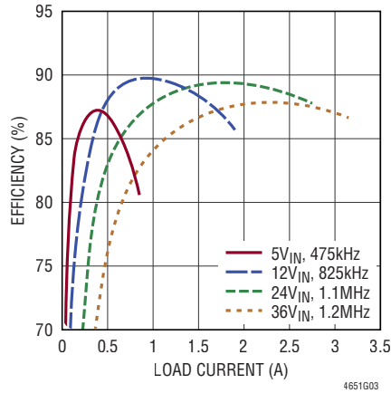
-12V Efficiency vs Load Current
