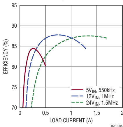
-24V Efficiency vs Load Current
