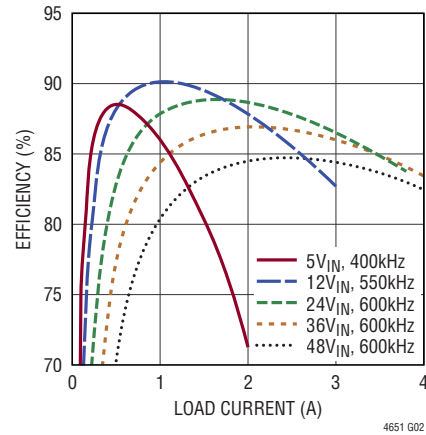
-5V Efficiency vs Load Current
