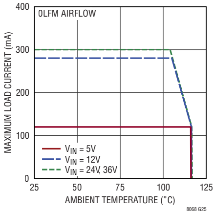
Derating, 1.8 V_{OUT2}
