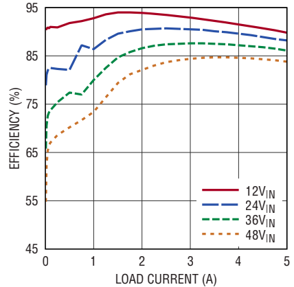
Efficiency vs Load Current V_{OUT} = 3.3\text{V} , \text{BIAS} = 5\text{V} , f_{SW} = 650\text{kHz}
