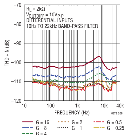
Total Harmonic Distortion + Noise vs Frequency
