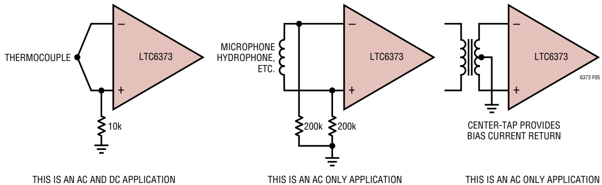
Figure 5. Providing an Input Common Mode Current Path
