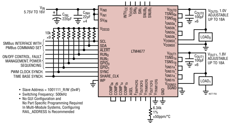
Figure 56. 18A, 1V and 18A, 1.8V Output DC/DC \mu Module Regulator with Serial Interface
