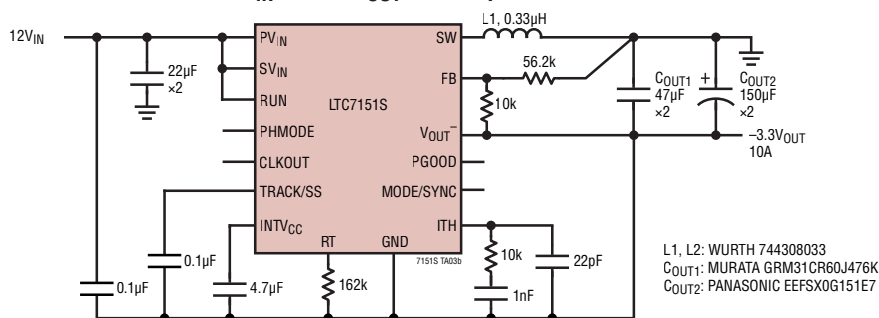
12VIN to -3.3VOUT 10A Step-Down Converter
