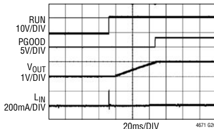
Start-Up Waveform with No Load Current Applied
