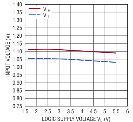
I 2 C SCL and SDA Input V IL and V IH vs V L Supply
