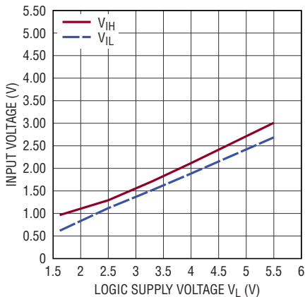
ON, CTRL, and REMOTE Inputs V IL and V IH vs V L Supply
