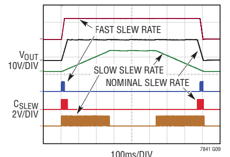
Output Voltage Changes with MFR_VOUT_COMMAND
