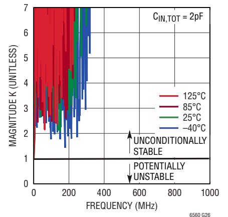
Stability Factor K vs Frequency Over Temperature
