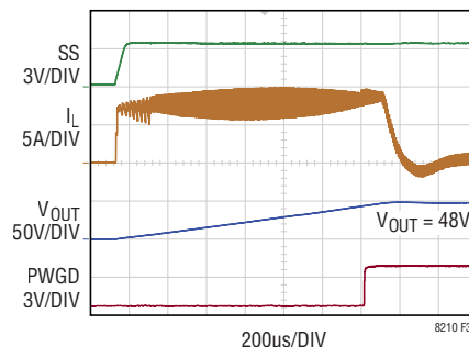
Figure 31. Typical Start-Up with No C_{SS}
