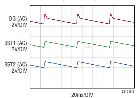
DG, BST1, BST2 Charging in Pass-Thru (Figure 36)
