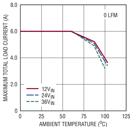
Derating, V_{OUT} = 1\text{V} BIAS = 5V, DC2860A Demo Board T_J = 120^\circ\text{C} , Burst Mode All Channels At Same Load
