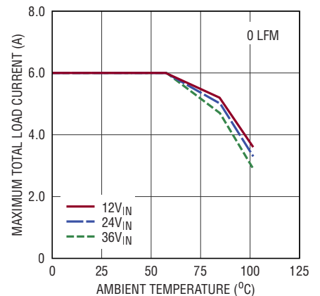
Derating, V_{OUT} = 1.2\text{V} BIAS = 5V, DC2860A Demo Board T_J = 120^\circ\text{C} , Burst Mode All Channels At Same Load
