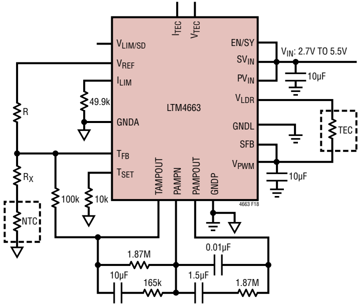
Figure 18. 2.7V to 5.5V Input, ±1.5A TEC Driver Circuit with Analog PID Compensation in a Temperature Control Loop
