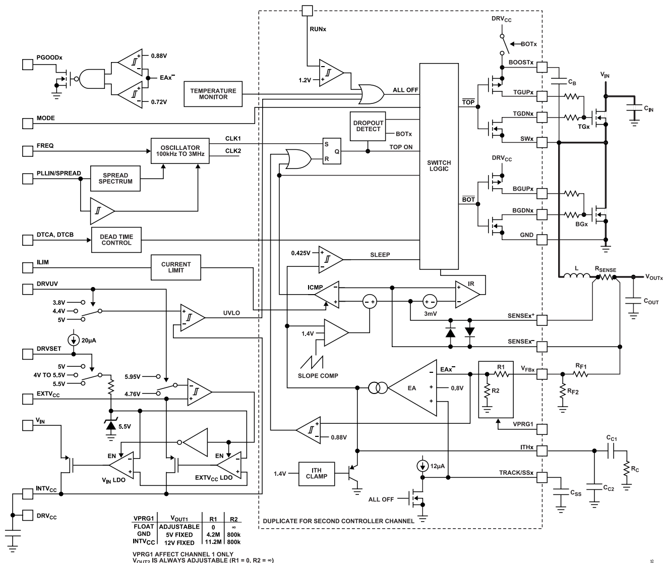
Figure 35. Functional Diagram
