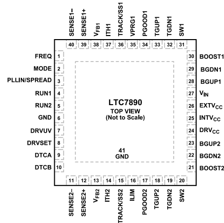
Figure 3. Pin Configuration
