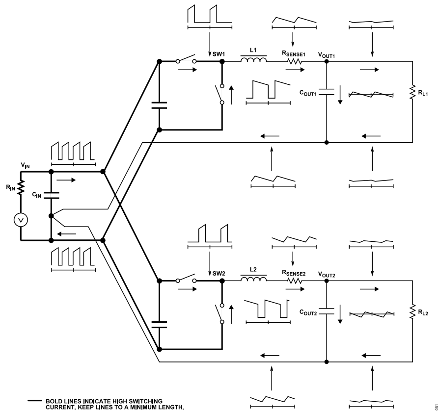
Figure 51. Branch Current Waveform
