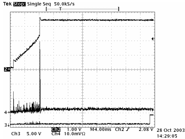
Figure 11. DC481 Soft Startup ( R_{LOAD} = 3.3\Omega , V_{IN} = 12V , V_{OUT} = 3.3V , T_A = 25^\circ C ) CH2 is V_{OUT} , CH3 is Power Good, CH4 is I_{IN} (200mA/10.0mV \Omega )
