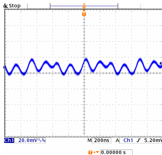
Figure 4. 1.5V Output Ripple ( V_{IN} = 3.3V , I_{OUT} = 600mA )
