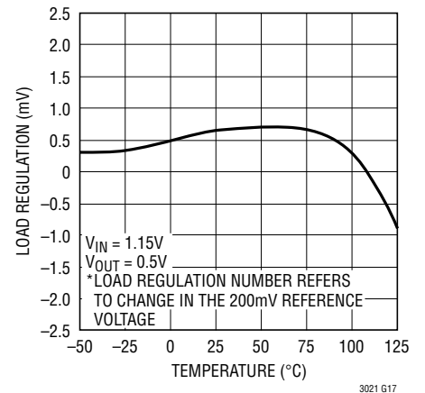
Load Regulation \Delta I_L = 1mA \text{ to } 500mA
