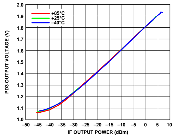
Figure 37. PD3 Output Voltage vs. IF Power Output at RF = 2 GHz, 56 MHz Filter
