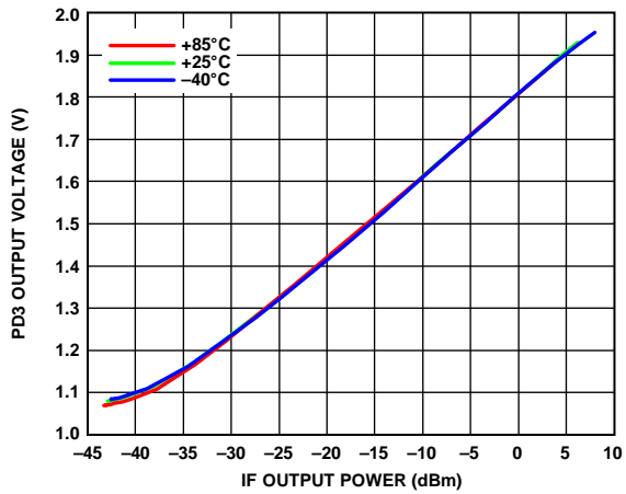
Figure 34. PD3 Output Voltage vs. IF Power Output at RF = 1 GHz, 56 MHz Filter
