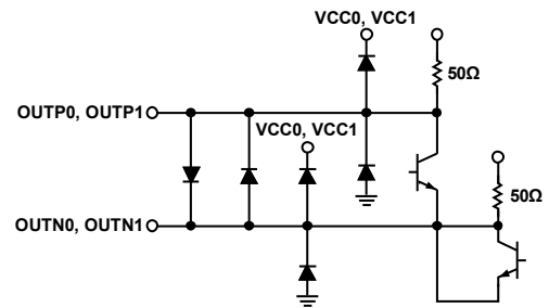
Figure 8. OUTPx, OUTNx Interface Schematic
