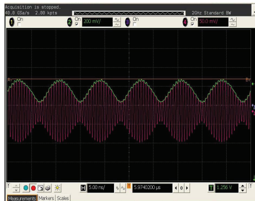
Figure 3. ETOU Response to an RF Input Signal with a 120 MHz Modulation Bandwidth
