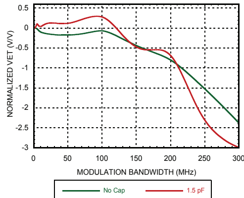
Figure 2. ETOU Bandwidth
