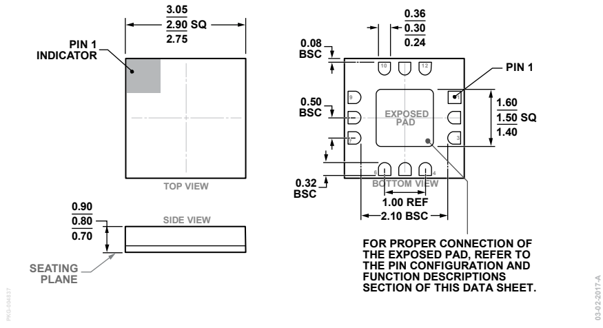
Figure 86. 12-Terminal Ceramic Leadless Chip Carrier (LCC) (E-12-4) Dimensions shown in millimeters
