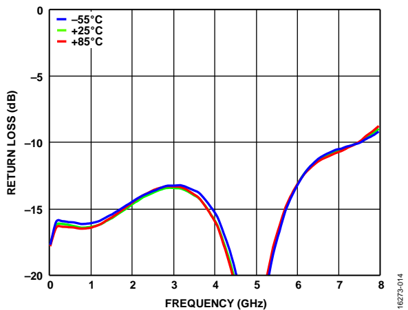
Figure 14. Input Return Loss vs. Frequency for Various Temperatures, Self Biased Mode, V_{DD} = 12\text{ V} , V_{GG1} = \text{GND} , V_{GG2} = \text{Open}
