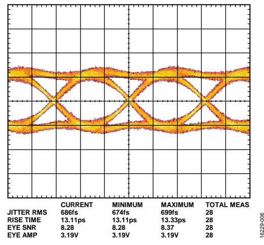
Figure 6. Differential Output, V_{CTL} = -1 V
