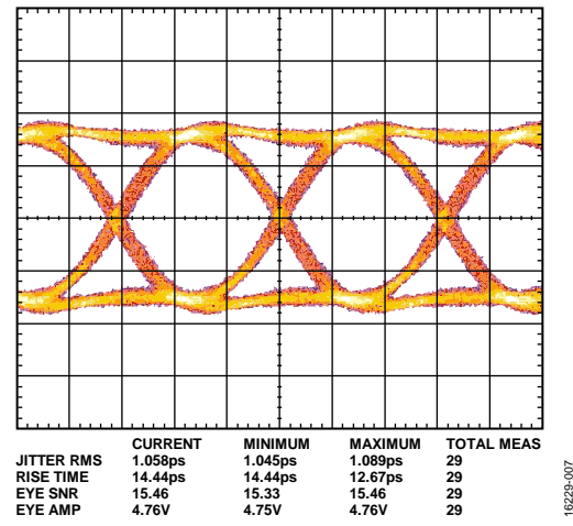
Figure 7. Differential Output, V_{CTL} = -1.5 V
