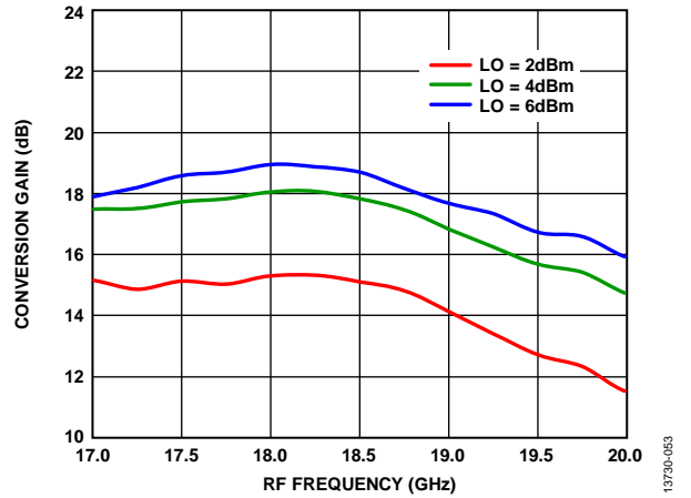
Figure 53. Conversion Gain vs. RF Frequency at Various LO Powers
