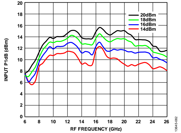
Figure 74. Input P1dB vs. RF Frequency at Various LO Drives, TA = 25°C
