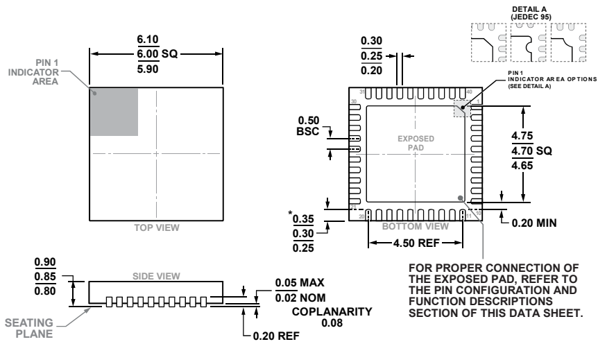
Figure 48. 40-Lead Lead Frame Chip Scale Package [LFCSPP] 6 mm × 6 mm Body and 0.85 mm Package Height (HCP-40-1)
