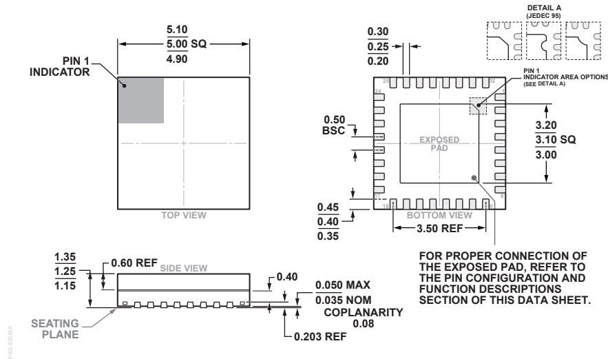
32-Lead Lead Frame Chip Scale Package, Premolded Cavity [LFCSP_CAV] 5 mm x 5 mm Body and 1.25 mm Package Height (CG-32-2) Dimensions shown in millimeters
