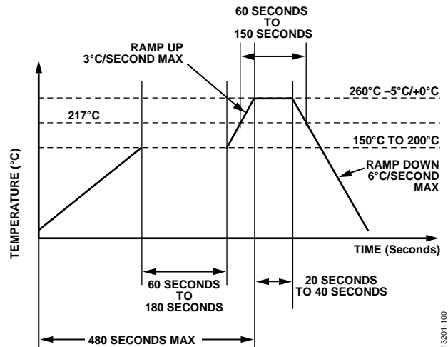
Figure 53. LFCSP Pb-Free Reflow Profile
