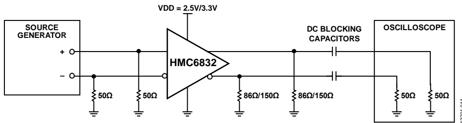
Figure 41. Test Circuit for Transient (AC) LVPECL Measurements, 86 Ω Termination Used for VDD = 2.5 V; 150 Ω Termination Used for VDD = 3.3 V
