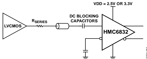
Figure 48. LVCMOS AC-Coupled Input Interface
