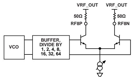
Figure 31. Output Stage
